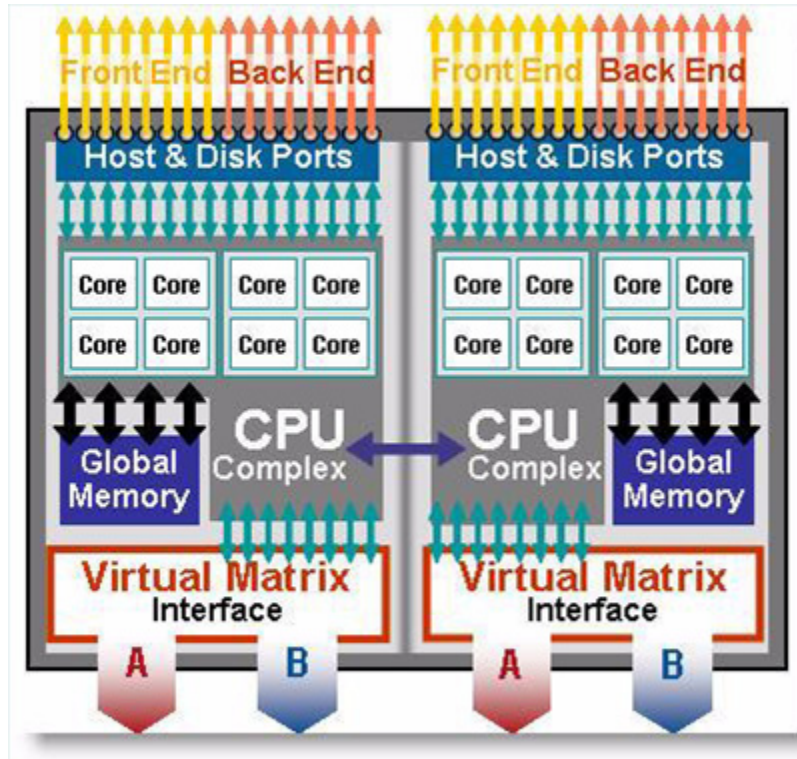
Figure 1 Symmetrix V-Max high availability node layout
