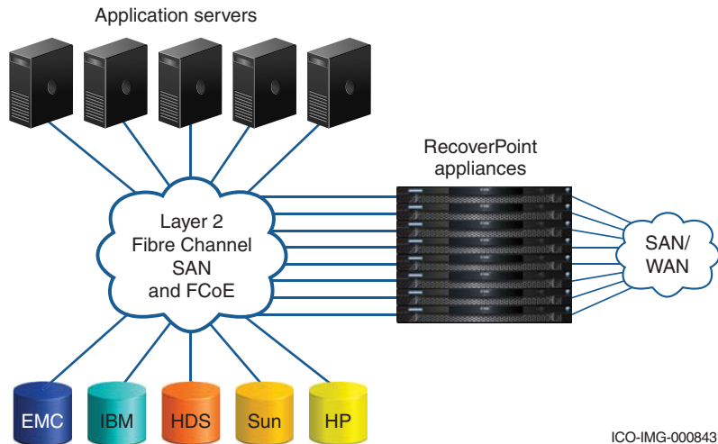
Figure 12 RecoverPoint architecture example
