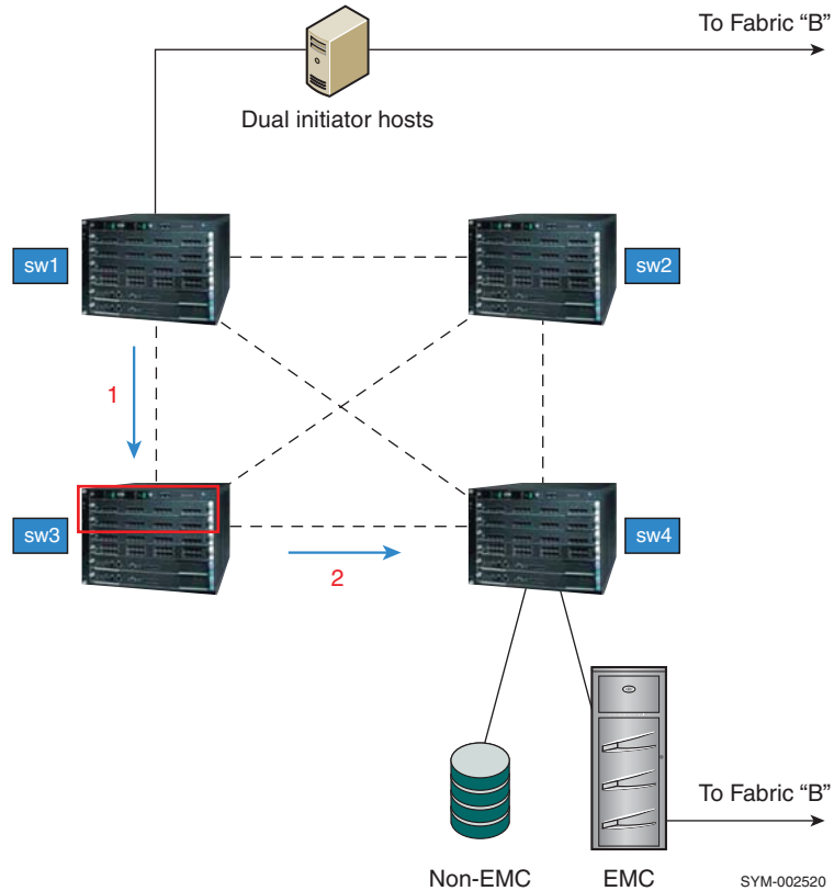
Figure 25 Four-switch mesh design using MDS 9506s (Example 1)
