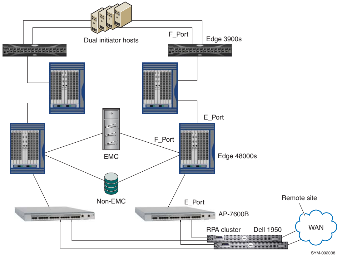
Figure 20 Core/edge design with a Connectrix B
