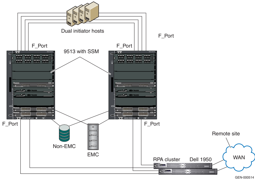
Figure 18 MDS 9513 with a 24-port line card and an SSM blade
