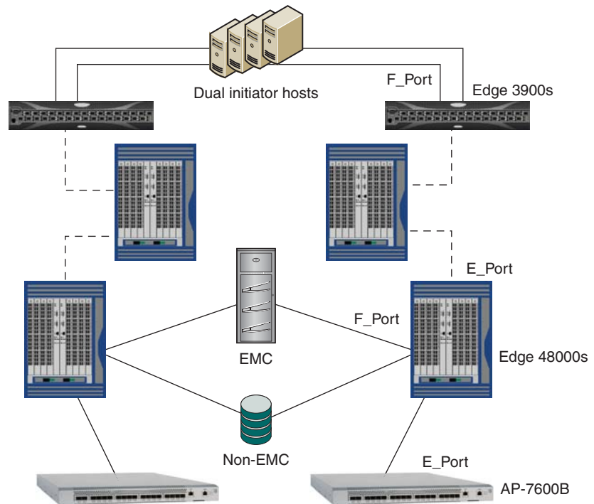
Figure 22 Core/edge/core design with Brocade
