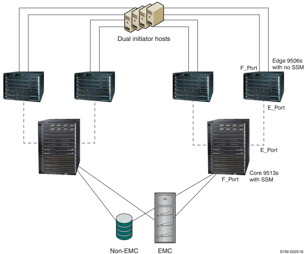
Figure 19 Core/edge design
