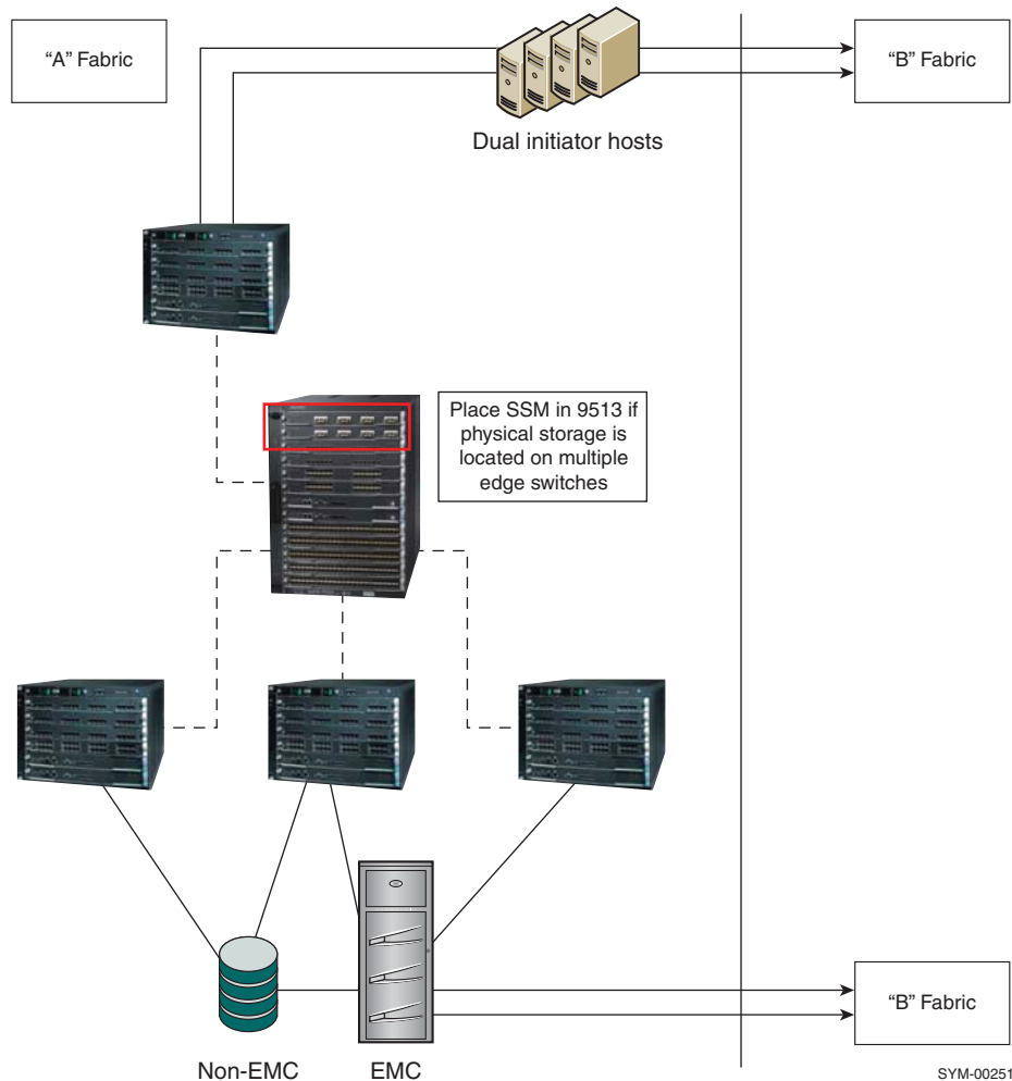
Figure 23 Storage on multiple switches
