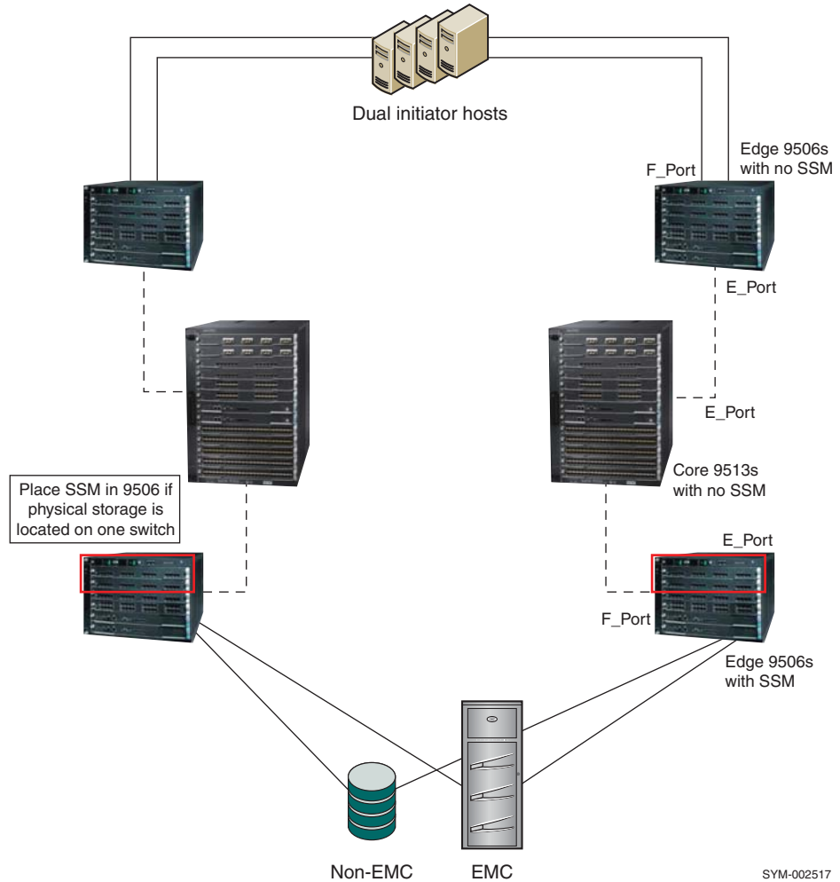
Figure 21 Storage on a single switch
