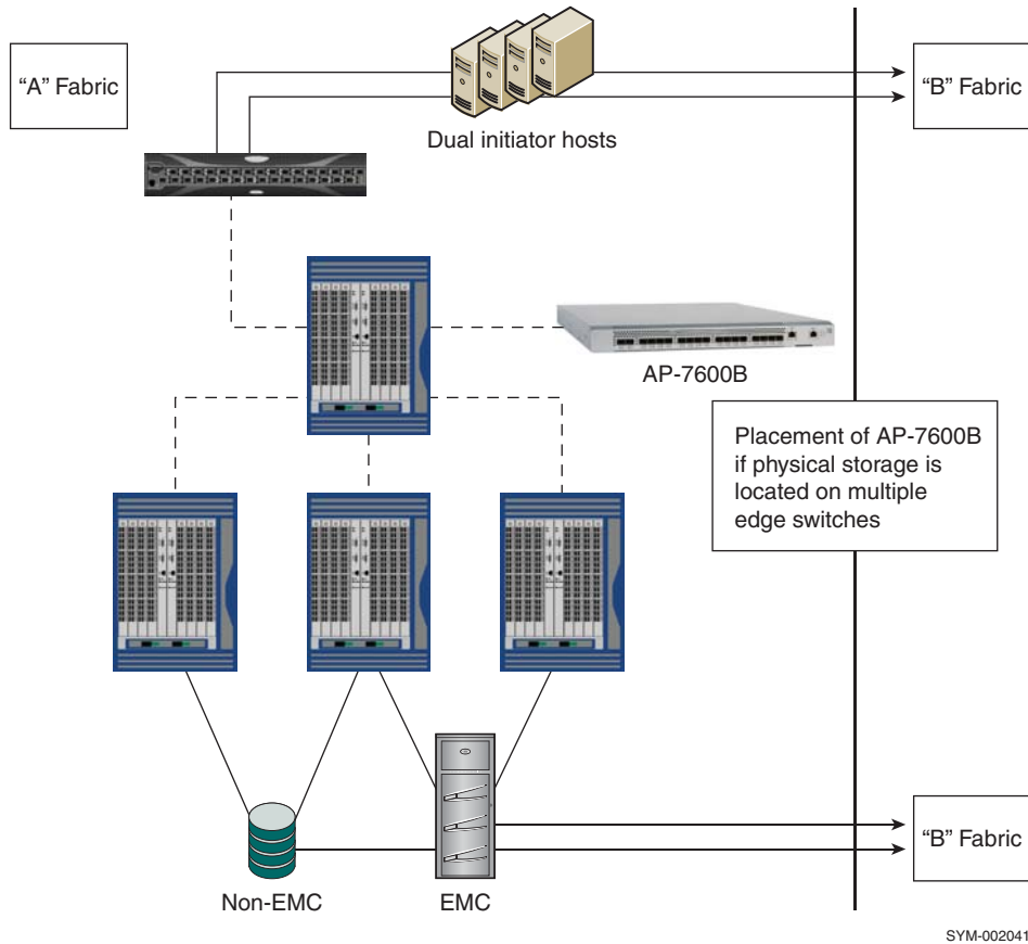
Figure 24 Storage on multiple switches with Connectrix B
