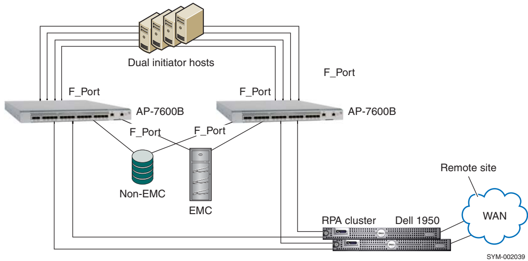
Figure 16 Connectrix B AP-7600B simple SAN topology
