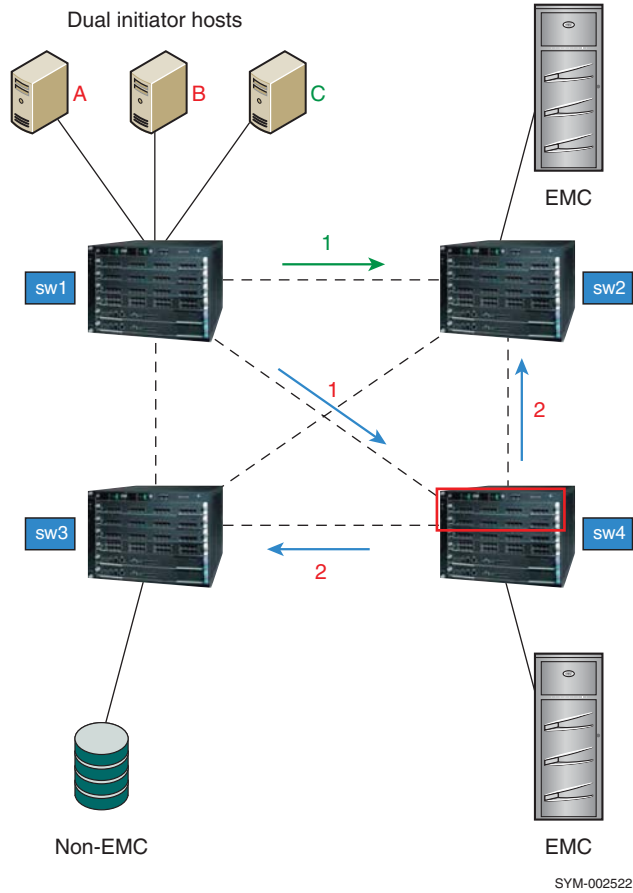
Figure 28 Four-switch mesh of MDS 9506s (Example 4)
