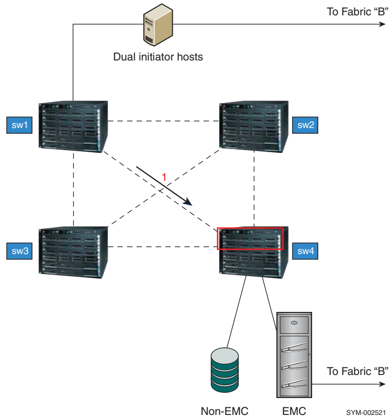
Figure 26 Four-switch mesh design using MDS 9506s (Example 2)
