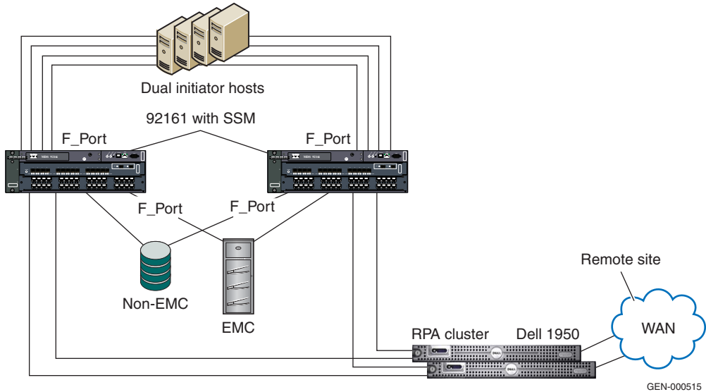
Figure 17 Connectrix MDS SSM blade in simple SAN topology
