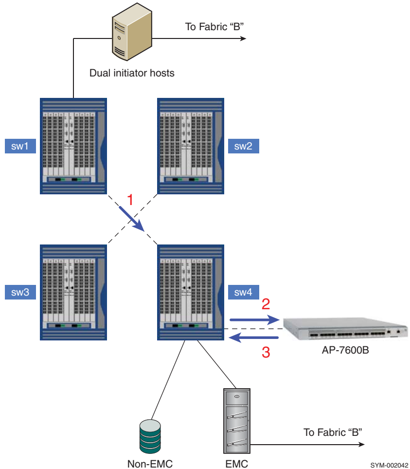
Figure 27 Four-switch mesh of ED-48000Bs with an AP-7600B as the intelligent switch (Example 3)
