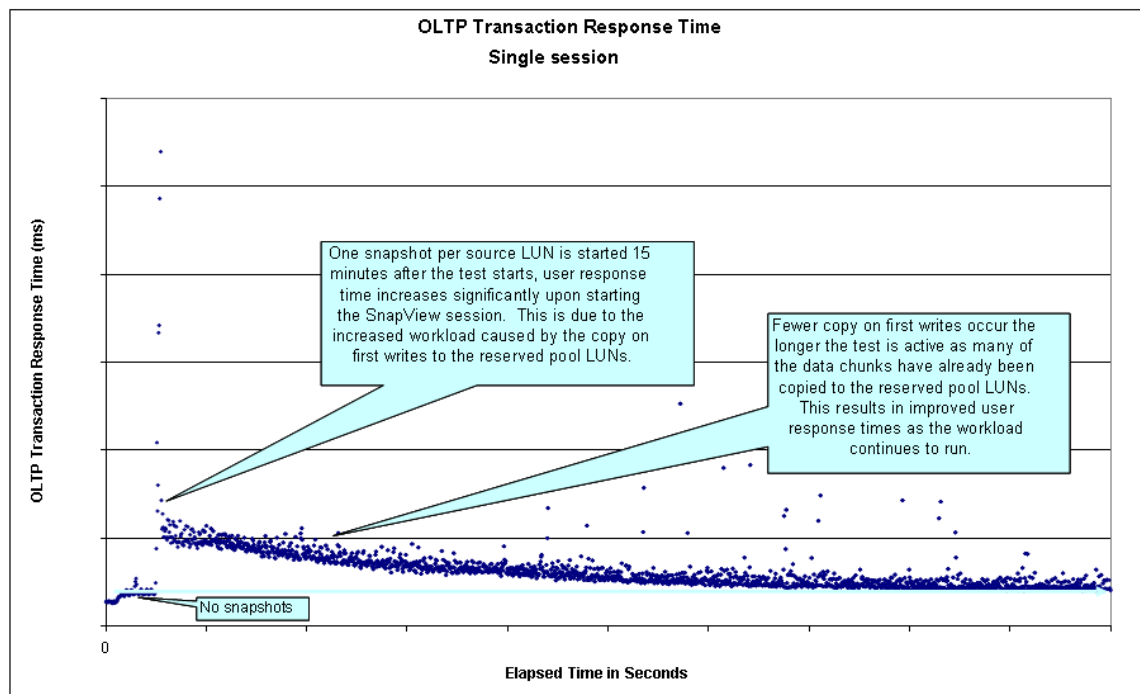
Figure 22. Response time during a single SnapView session
