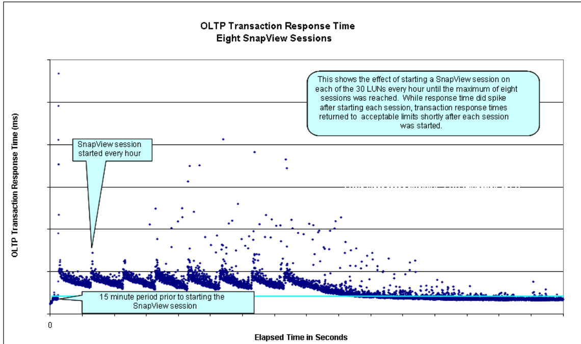
Figure 23. Response time during multiple SnapView sessions
