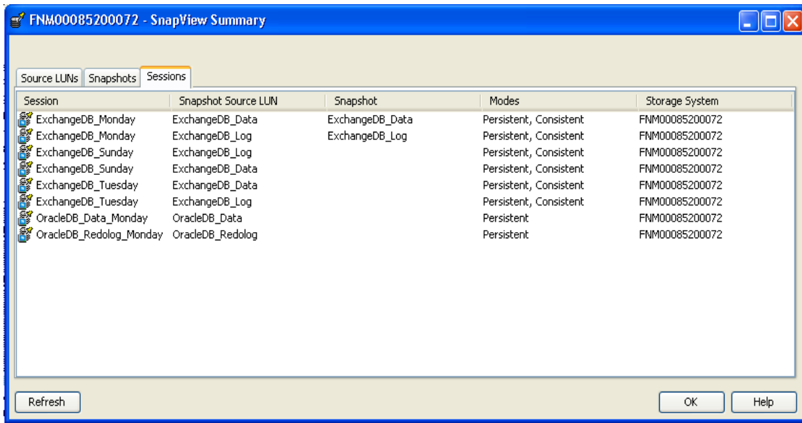
Figure 10. SnapView summary
