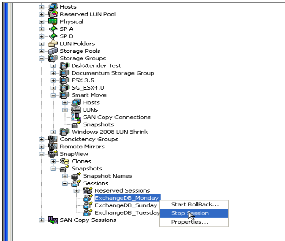
Figure 13. Stopping sessions
