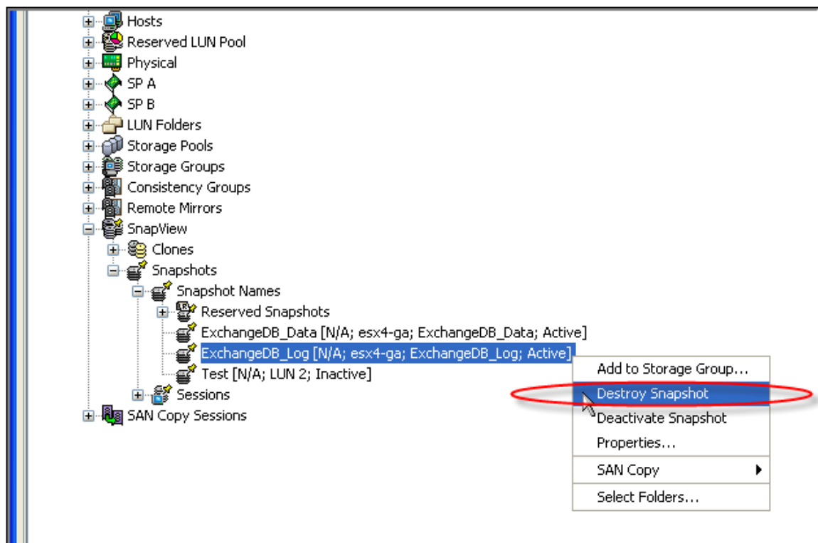
Figure 12. Destroying snapshots
