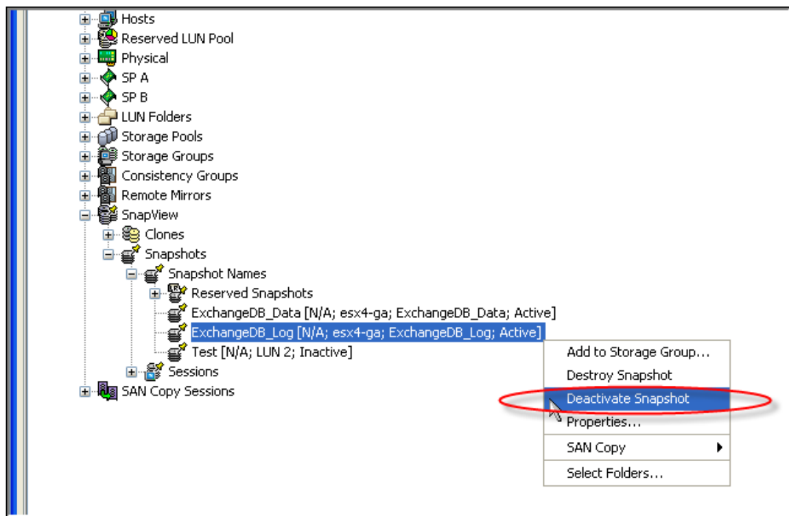
Figure 11. Deactivating snapshots
